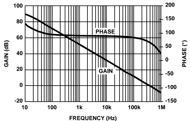
FIGURE 16. AMPLIFIER "B" (OP-AMP) A_{VOL} vs FREQUENCY @ 1kΩ LOAD
