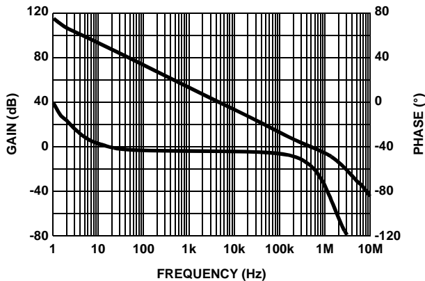
FIGURE 15. AMPLIFIER "B" (OP-AMP) A_{VOL} vs FREQUENCY @ 100kΩ LOAD
